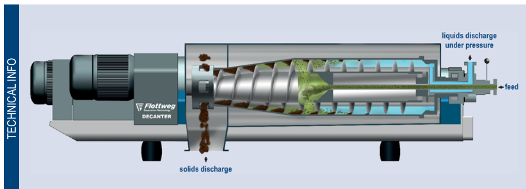
Flottweg Decanter with pressurized centrate discharge
